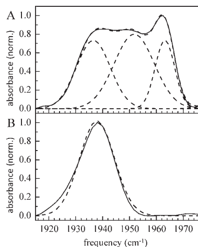
Figure 2. Linear FT IR spectra (—), along with the Gaussian fits (---) to the spectra, of (A) substrate-free cyt P450 cam –CO and (B) its complex with camphor.
